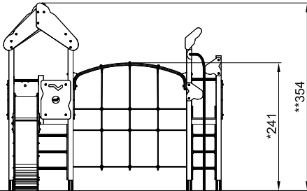
BASIC811100P 1:100
