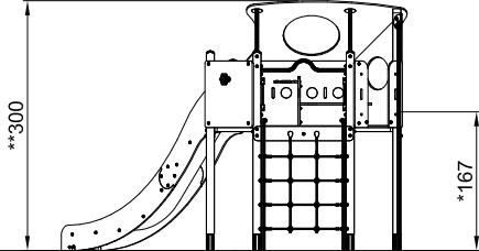
MQS100100P 1:100
